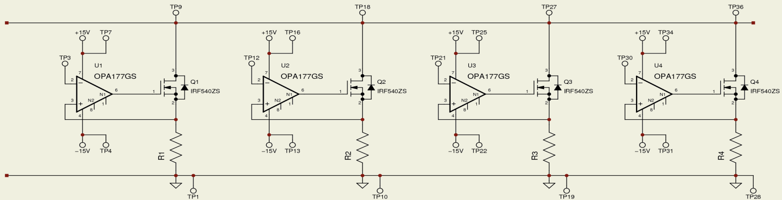
Figure 2: Load Schematic
