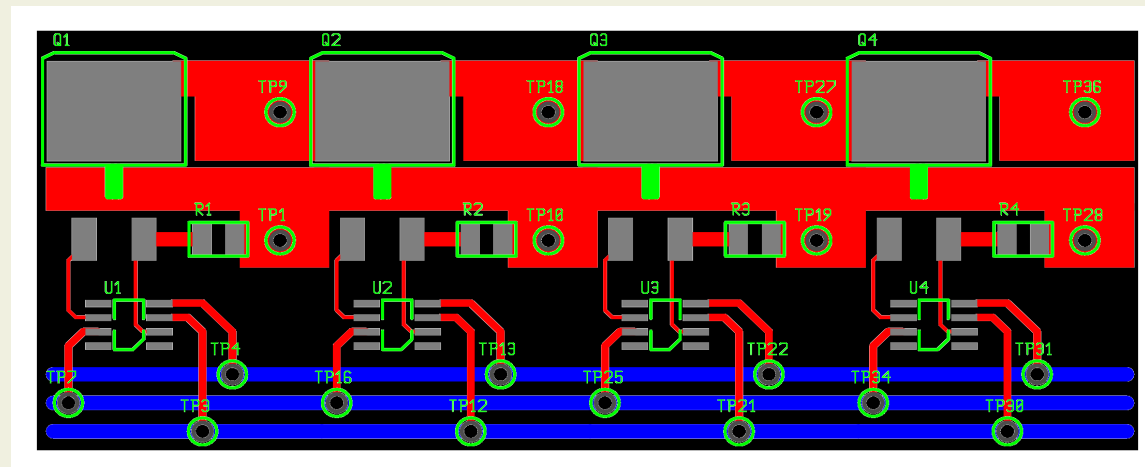
Figure 4: Load PCB
